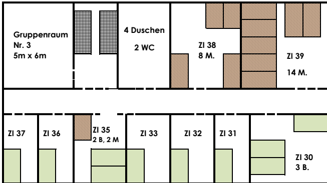
3. Stock
